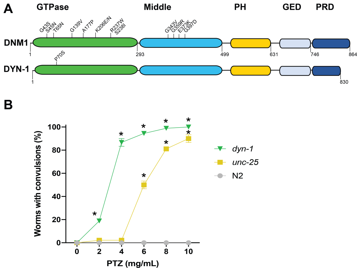
Figure 1. Modeling convulsions associated with human DNМ1 encephalopathy: (A) Schematic comparison of human DNМ1 and C. elegans DYN-1. The domains present in the proteins are shown and include the GTPase domain which is involved in GTP binding and hydrolysis, the middle domain, a GTPase effector domain (GED) required for oligomerization and stimulation of GTPase activity, the pleckstrin homology (PH) domain, and a proline-rich domain (PRD). Mutations associated with seizures in humans are indicated in the GTPase and middle domains of DNM1 . A temperature-sensitive missense mutation in C. elegans , dyn-1(ky51) , is located in the GTPase domain. (B) PTZ induces convulsions in C. elegans dyn-1(ky51) and a positive control mutant, unc-25(e156) , in a dose-responsive manner, while N2 worms do not respond to this chemical. * p < 0.0001 Two-Way ANOVA with a Dunnett's post-hoc analysis where dyn-1(ky51) is compared to N2 and unc-25(e156) is compared to N2.
